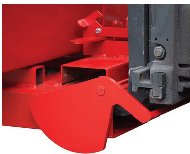
Forks locking mechanism
